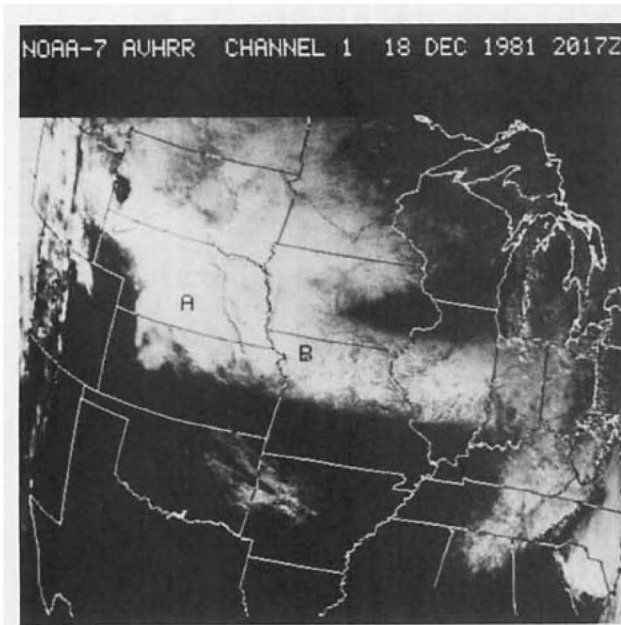
FIG. 2. 0.6 \mu\text{m} AVHRR image.
