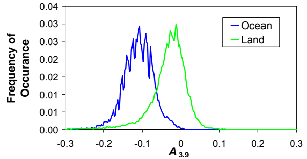
Figure 5. Histograms of A_{3.9} over land and ocean. Over land the mean is -0.032 and the standard deviation is 0.049 . Over ocean the mean is -0.110 and the standard deviation is 0.040 .
