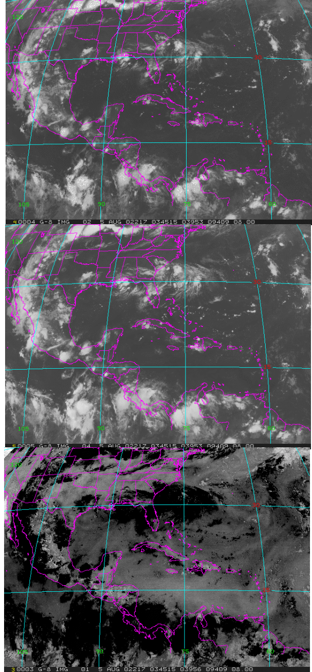
Figure 1. Nighttime example: (top) 3.9 \mu\text{m} image, (middle) 10.7 \mu\text{m} image, (bottom) 3.9 \mu\text{m} albedo.
