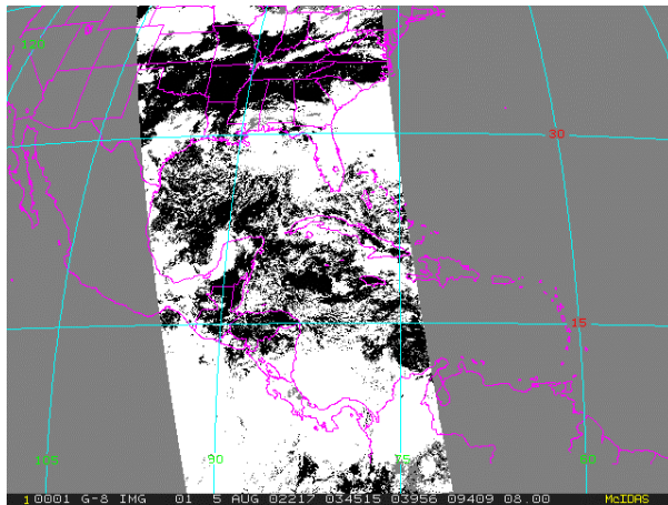
Figure 4. MODIS cloud mask corresponding to Fig. 1. White indicates cloud, black indicates clear, and gray indicates uncertain classification or not observed.
