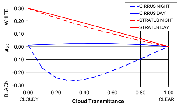
Figure 3. A_{3.9} calculated for transmissive stratus and cirrus clouds. See text for model details.
