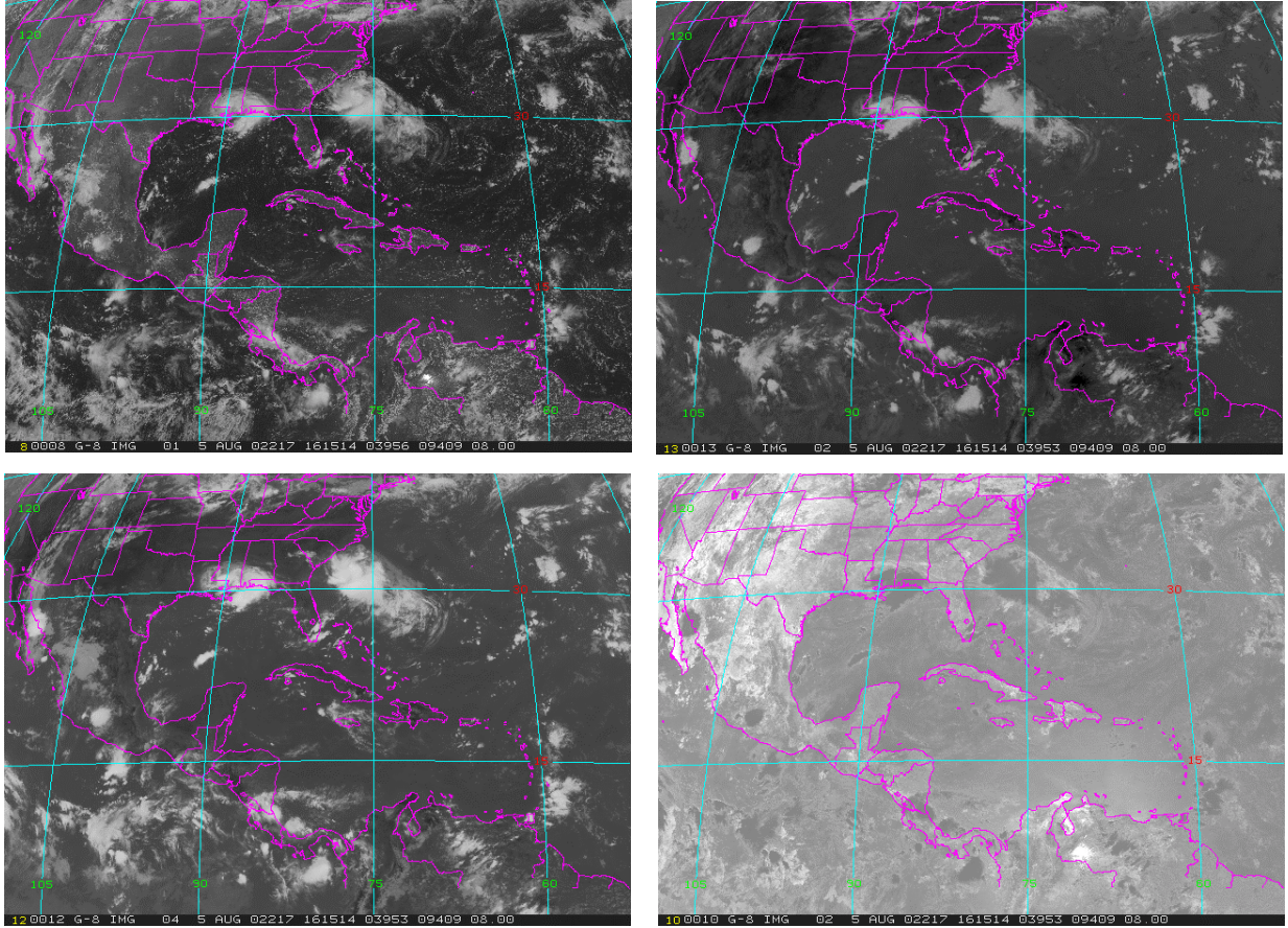
Figure 2. Daytime example: (top left) 0.64 \mu\text{m} albedo, (top right) 3.9 \mu\text{m} image, (bottom left) 10.7 \mu\text{m} image, (bottom right) 3.9 \mu\text{m} albedo.
