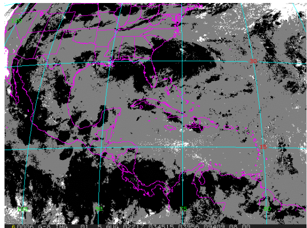
Figure 6. GOES A_{3.9} nighttime cloud mask. Black is cirrus, white is stratus, and gray is clear.
